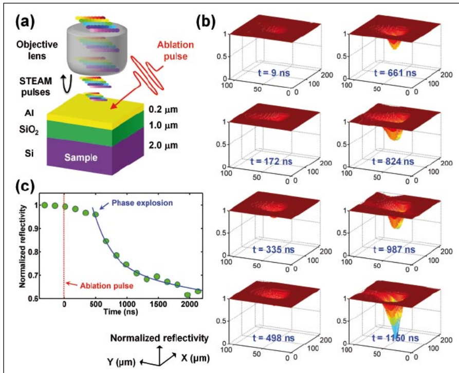
FIGURE 3: Observation of laser ablation dynamics with STEAM. (a) Schematic of the experiment. (b) Real-time STEAM images of the laser ablation dynamics at a frame rate of 6.1 MHz corresponding to a frame repetition period of 163 ns with 440 ps shutter speed. (c) Evolution of the normalized reflectivity map of the sample that indicates the phase explosion effect.
