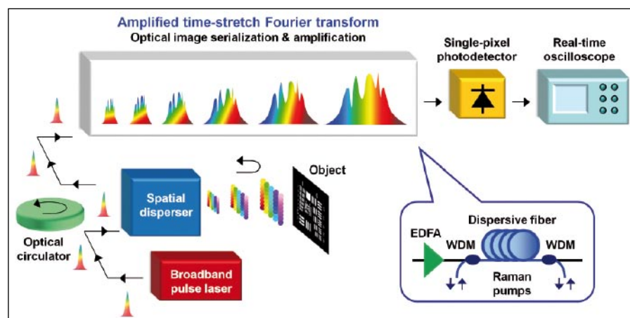
FIGURE 2: Serial time-encoded amplified microscopy (STEAM).
