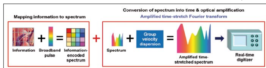
FIGURE 1: Concepts of spectral encoding and amplified time-stretch Fourier transform.
