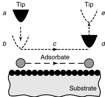
Figure A.7 Schematic of the sliding process: a and e —imaging, b —connecting, c —sliding, d —disconnecting.
