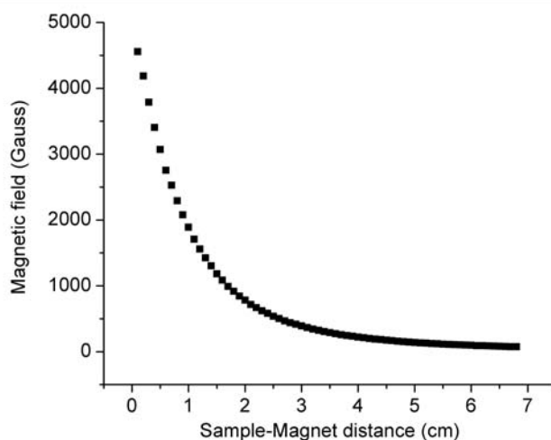
Figure SI-1. Dependence of strength of the magnetic field to the sample-magnet distance for the NdFeB magnet used in the experiments.
