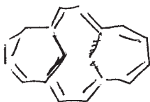
[16] annulene with E Vogel
